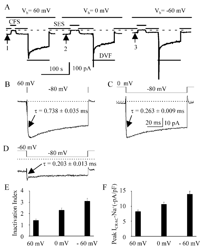
FIGURE 7 Ca^{2+} binding to the potentiation site is voltage dependent. (A) Currents were detected by 80-ms voltage steps of -80 mV from a holding potential ( V_h ) of 60, 0, or -60 mV. The current values at 70 ms after the initiation of the -80 mV voltage steps are displayed. The V_h values labeled above the horizontal bars indicate the holding potential between the -80 mV voltage steps. (B, C, and D) The averaged currents invoked by the indicated voltage steps, taken around the points labeled by arrows 1 ( n = 14 ), 2 ( n = 12 ), and 3 ( n = 10 ) in panel A, respectively. (E) Inactivation index of Na^+-I_{CRAC} when V_h = 60 , 0, or -60 mV, n = 5 for all cases. (F) The peak Na^+-I_{CRAC} when V_h = 60 , 0, or -60 mV, n = 5 for all cases.
