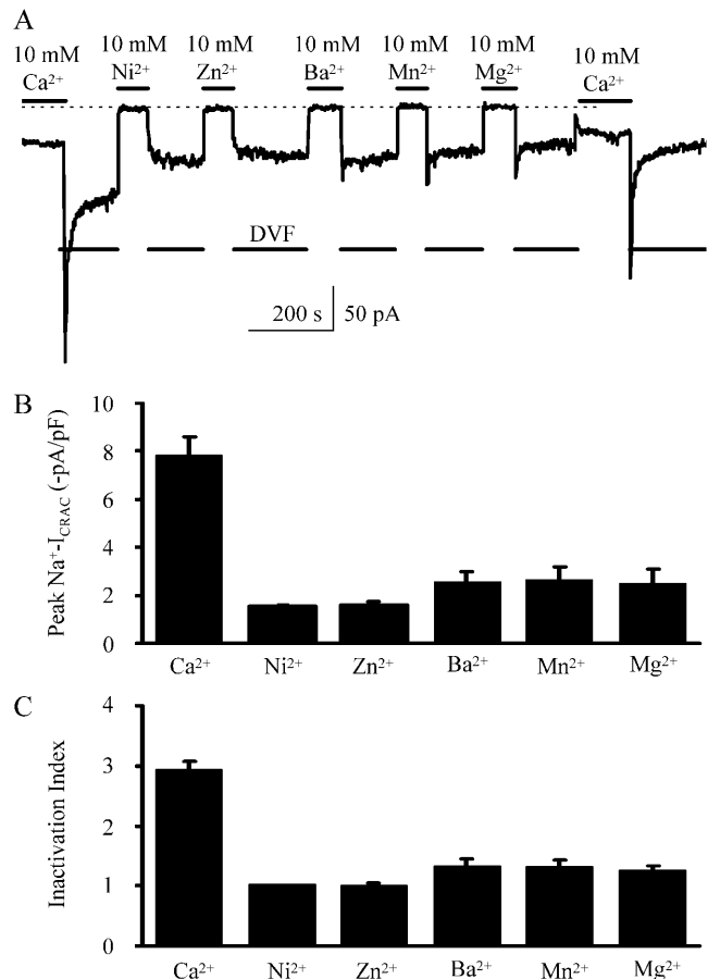
FIGURE 3 \text{Ca}^{2+} dissociation from a site on the CRAC channel is responsible for the inactivation of \text{Na}^+ - I_{\text{CRAC}} . (A) Preexposing a cell to 10 mM \text{Ca}^{2+} (the solution contained (in mM) 149 N -methyl-D-glutamine chloride, 10 \text{CaCl}_2 , 5 D-glucose, and 10 HEPES) greatly potentiated \text{Na}^+ - I_{\text{CRAC}} that inactivated rapidly. Preexposing the cell to 10 mM \text{Ni}^{2+} or \text{Zn}^{2+} (replacing \text{CaCl}_2 by equal-molar \text{NiCl}_2 or \text{ZnCl}_2 in the above solution) failed to potentiate the \text{Na}^+ - I_{\text{CRAC}} . Preexposing the cell to 10 mM \text{Ba}^{2+} or \text{Mn}^{2+} or \text{Mg}^{2+} (replacing \text{CaCl}_2 by equal-molar \text{BaCl}_2 , \text{MnCl}_2 , or \text{MgCl}_2 in the above solution) only partially potentiated the \text{Na}^+ - I_{\text{CRAC}} . Reexposing the cell to 10 mM \text{Ca}^{2+} restored the potentiation. (B) The peak \text{Na}^+ - I_{\text{CRAC}} when cells were preexposed to 10 mM \text{Ca}^{2+} ( n = 7 ), \text{Ni}^{2+} ( n = 6 ), \text{Zn}^{2+} ( n = 6 ), \text{Ba}^{2+} ( n = 7 ), \text{Mn}^{2+} ( n = 6 ), or \text{Mg}^{2+} ( n = 7 ). (C) The inactivation indices of \text{Na}^+ - I_{\text{CRAC}} when cells were preexposed to 10 mM \text{Ca}^{2+} ( n = 7 ), \text{Ni}^{2+} ( n = 6 ), \text{Zn}^{2+} ( n = 6 ), \text{Ba}^{2+} ( n = 7 ), \text{Mn}^{2+} ( n = 6 ), or \text{Mg}^{2+} ( n = 7 ).
