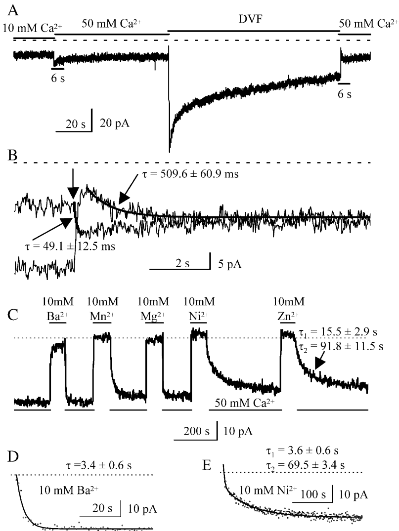
FIGURE 6 Ca 2+ binding to the potentiation site is required for the functioning of CRAC channels. (A) I_{CRAC} of a cell preexposed to 10 mM Ca 2+ increased rapidly when the extracellular Ca 2+ concentration was increased to 50 mM. However, when the cell was preexposed to DVF, subsequent exposing the cell to 50 mM Ca 2+ rapidly inhibited Na + - I_{CRAC} , which was then followed by a slow increase in Ca 2+ - I_{CRAC} . Solutions containing 10 or 50 mM Ca 2+ were made by adding the required CaCl 2 to a solution containing (in mM): 149 or 89 N -methyl-D-glutamine (NMDG) chloride, respectively, as well as 5 D-glucose, and 10 HEPES. (B) The two segments of current (6-s long) indicated by the horizontal bars labeled "6 s" in panel A are superimposed and displayed on an expanded timescale. The vertical arrow indicates the initiation of the solution exchange. The smooth lines are the fitted curves for current development ( n = 6 ). (C) Preexposing the cell to 10 mM Ba 2+ , Mn 2+ , or Mg 2+ partially potentiated Ca 2+ - I_{CRAC} , whereas Ni 2+ and Zn 2+ did not. (D) The time course of Ca 2+ - I_{CRAC} development when the cell was preexposed to 10 mM Ba 2+ (taken from panel C), is shown on an expanded timescale. (E) The time course of Ca 2+ - I_{CRAC} development when the cell was preexposed to 10 mM Ni 2+ (taken from panel C), is shown on an expanded timescale.
