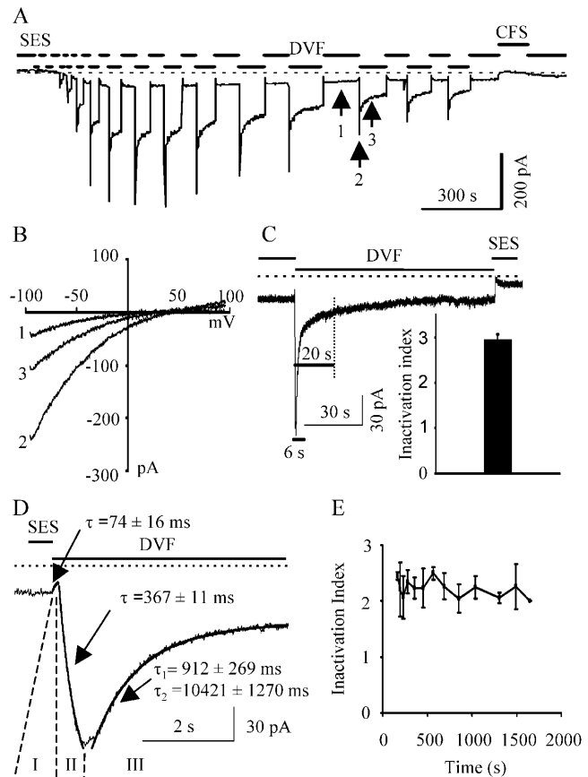
FIGURE 1 Inactivation of \text{Na}^+ - \text{I}_{\text{CRAC}} . (A) Whole-cell break-in on an RBL-2H3 cell activated \text{Ca}^{2+} - \text{I}_{\text{CRAC}} and \text{Na}^+ - \text{I}_{\text{CRAC}} when the external solution was alternated between standard extracellular solution (containing (in mM) 143 NaCl, 10 \text{CaCl}_2 , 1 \text{MgCl}_2 , 5 D-glucose, 4.5 KCl, 0.5 \text{BaCl}_2 , and 10 HEPES) and divalent-free solution (containing (in mM) 160 Na-methane sulphonate, 5 D-glucose, 2 Na-EGTA, and 10 HEPES). The current was detected by applying voltage ramps at 1 Hz and the values at -80 are displayed. Note that \text{Ca}^{2+} -free solution (containing (in mM) 143 NaCl, 11 \text{MgCl}_2 , 5 D-glucose, 4.5 KCl, 0.5 \text{BaCl}_2 , and 10 HEPES) completely abolished the \text{I}_{\text{CRAC}} . The horizontal dotted lines represent 0 current level in this and the following figures. (B) The I-V relationships of the current taken at the corresponding number-labeled time points in panel A when it reached steady state of \text{Ca}^{2+} - \text{I}_{\text{CRAC}} (trace 1), peak of \text{Na}^+ - \text{I}_{\text{CRAC}} (trace 2), and steady state of \text{Na}^+ - \text{I}_{\text{CRAC}} (trace 3). (C) The current from another cell was continuously recorded under -60 mV to reveal the fast kinetics of the transient current during the solution exchange. (inset) The inactivation index (see text for definition) of the \text{Na}^+ - \text{I}_{\text{CRAC}} when the extracellular solution was exchanged from SES to DVF, n = 16 . (D) The segment of the current (6-s long) as indicated by the horizontal bar near the peak of the current in panel C is displayed on an expanded timescale, revealing a three-phase kinetics of the current during the solution exchange. The smooth lines are the fitting curves for the preactivation (I), activation (II), and inactivation (III) phases of the \text{Na}^+ - \text{I}_{\text{CRAC}} , n = 16 . (E) Inactivation index of \text{Na}^+ - \text{I}_{\text{CRAC}} as a function of time after whole-cell break-in. Data are pooled from experiments as in panel A, n = 4 .
